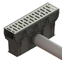
Conexiune teava DN50, 75, 110
