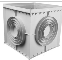
Camin PP BASE patrat Gri tip I A15-C250 550x550 (551I-G)
