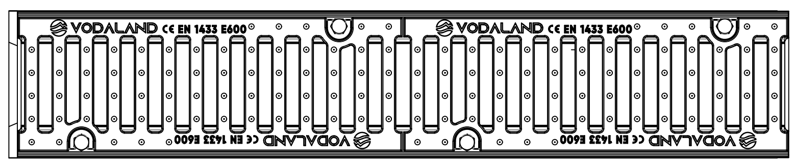
Channel with Grate E600 Channel with Grate E600 and vertical outlet 110
